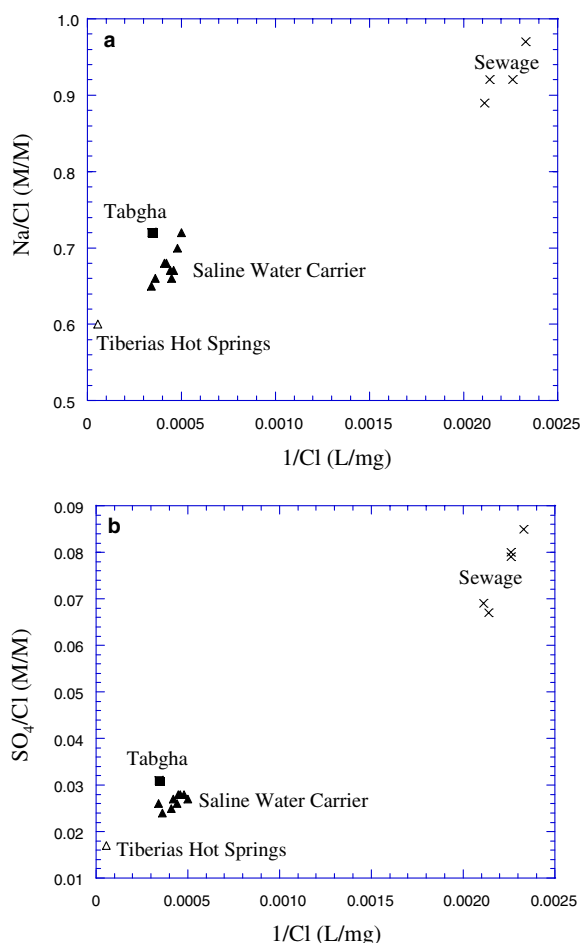
Fig. 4. Na/Cl (a) and \text{SO}_4/\text{Cl} (b) versus 1/\text{Cl} (L/mg) of the saline water springs (i.e., Tabgha and Tiberias Hot Springs) sewage water (as sampled at Bitaniya) and the Saline Water Carrier (SWC; as sampled below the Alumot Dam). Note that the salt content of the SWC is controlled by the chemical composition of the Tiberias Hot Springs and not the Tabgha Springs.
